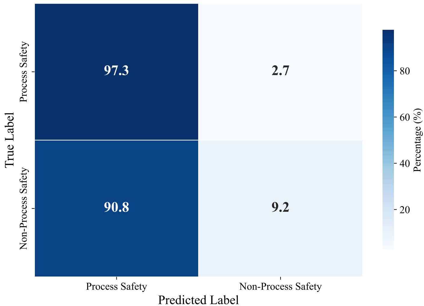
Normalised Confusion Matrix — Swedish (XLM-RoBERTa XNLI)
