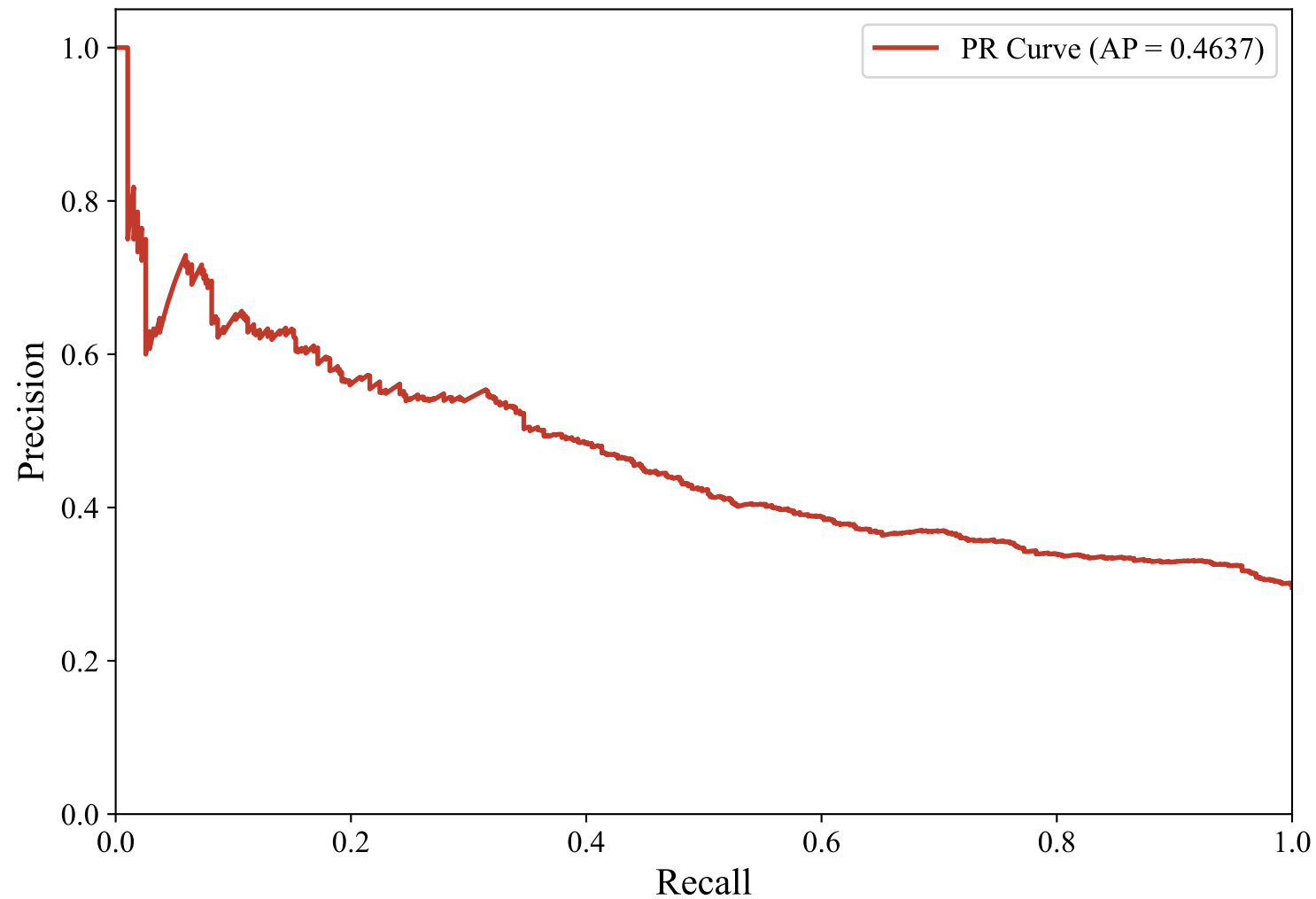
Precision-Recall Curve — Dutch (XLM-RoBERTa XNLI, Zero-Shot)
