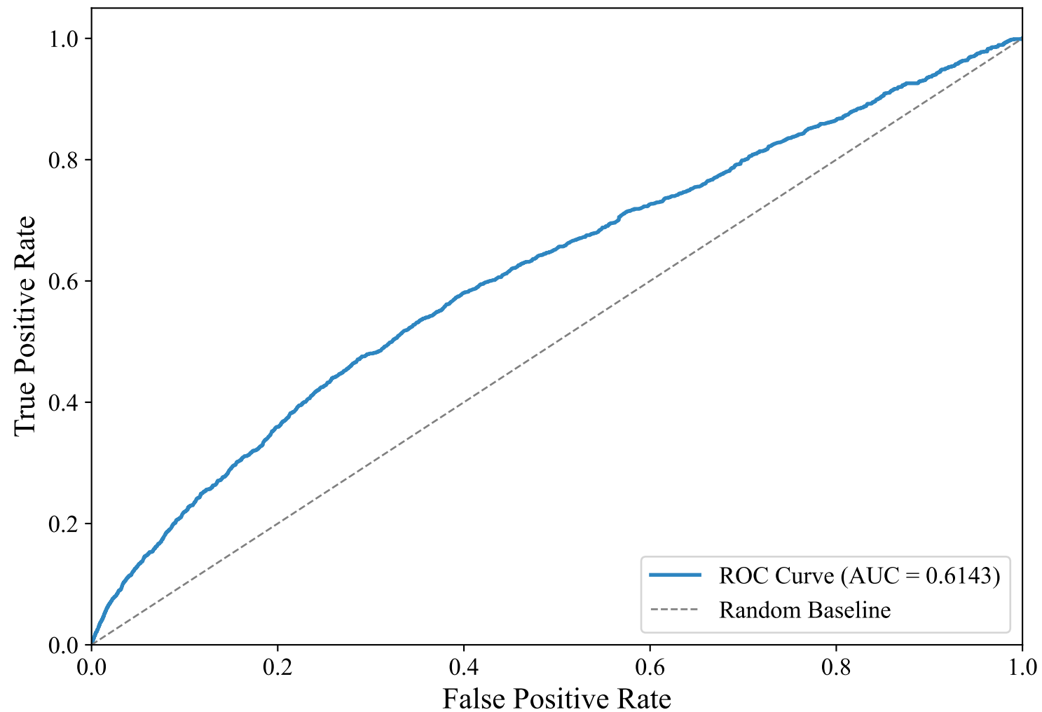
ROC Curve — German (XLM-RoBERTa XNLI, Zero-Shot)
