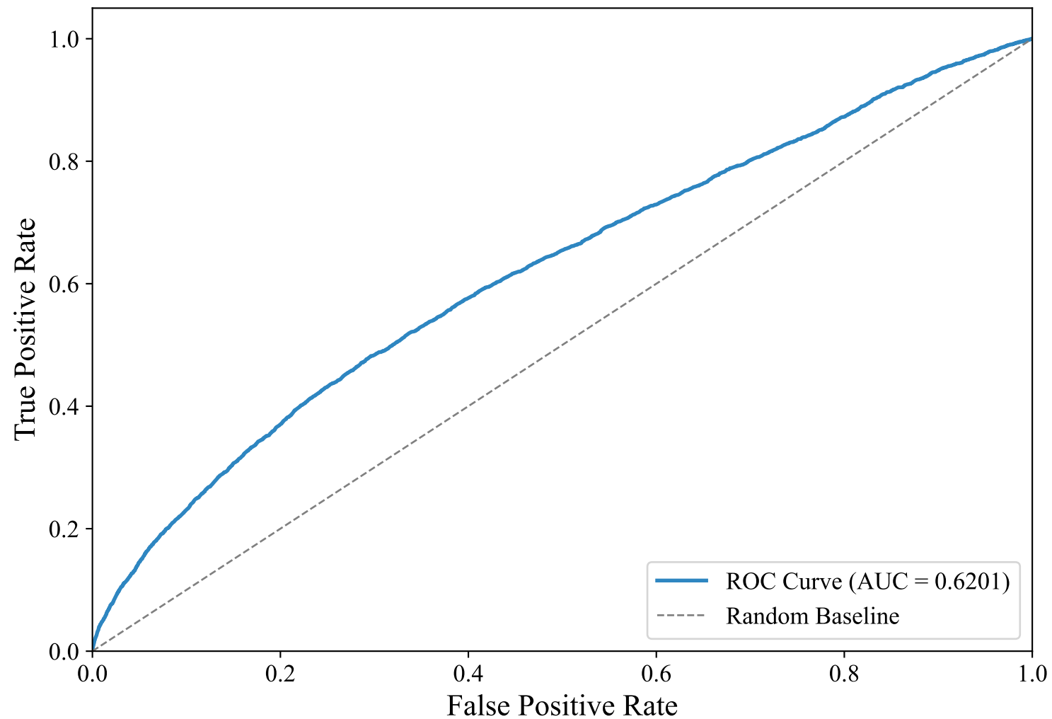
ROC Curve — Overall (XLM-RoBERTa XNLI, Zero-Shot)
