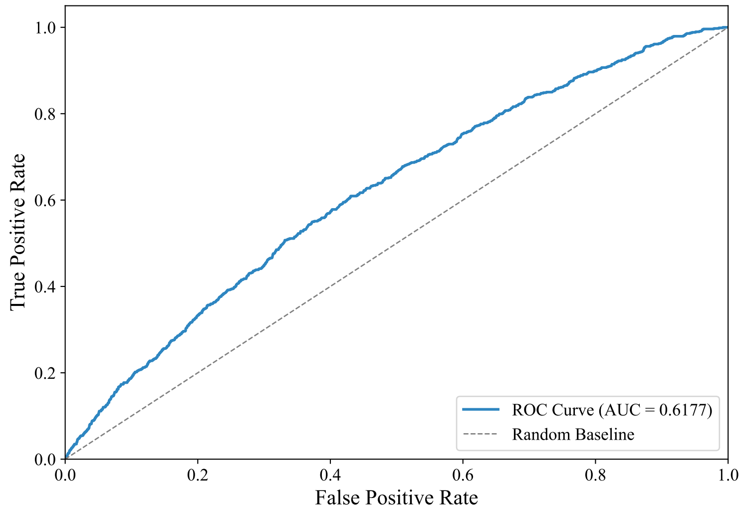
ROC Curve — Swedish (XLM-RoBERTa XNLI, Zero-Shot)
