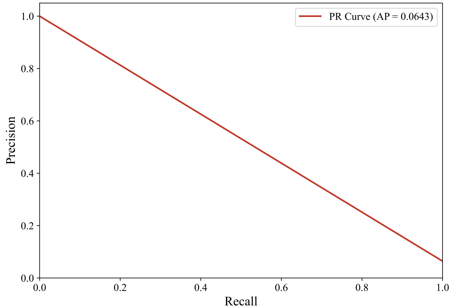
Precision-Recall Curve — Swedish (flan-t5-large, Few-Shot)
