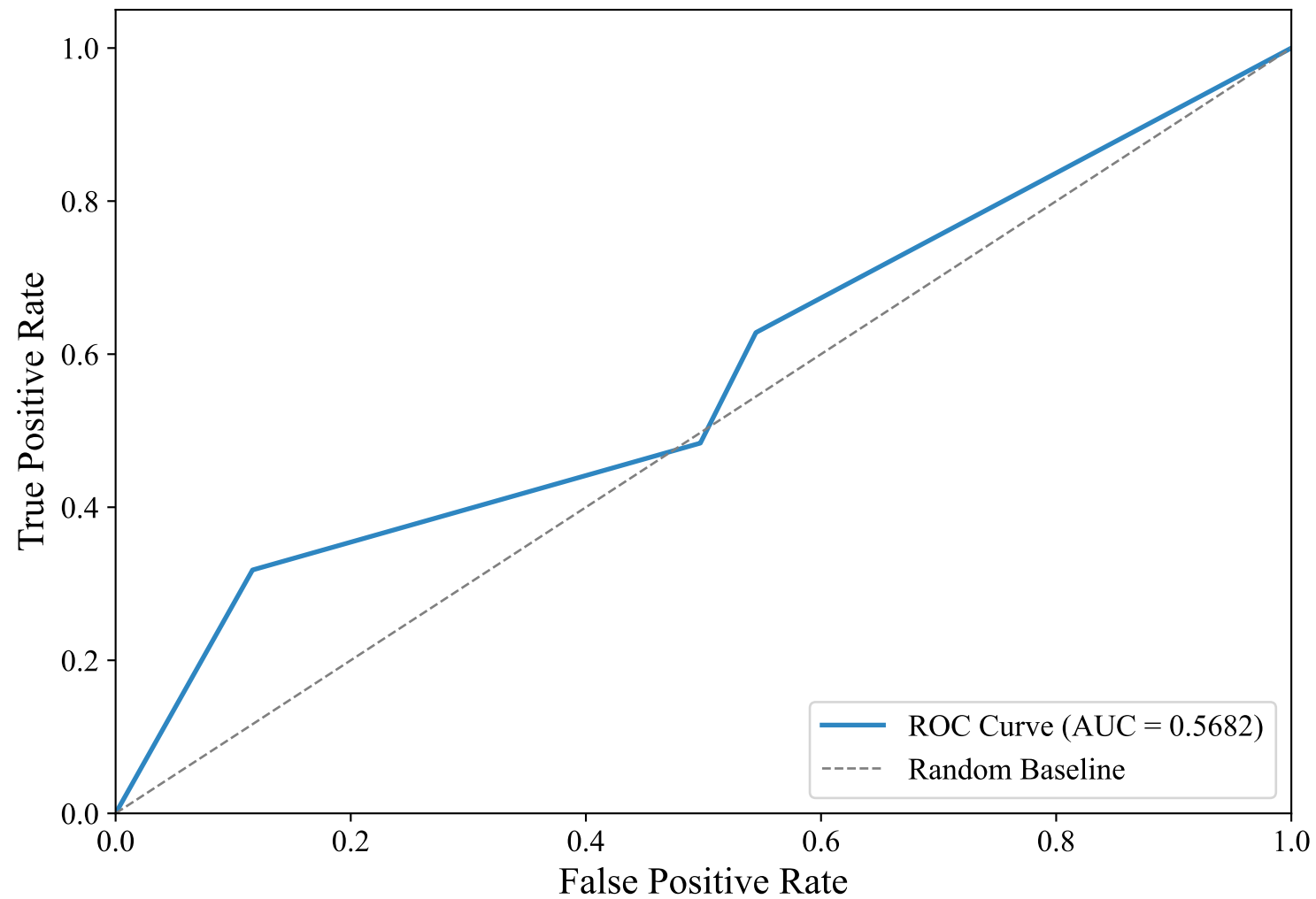
ROC Curve — Overall (flan-t5-large, Few-Shot)
