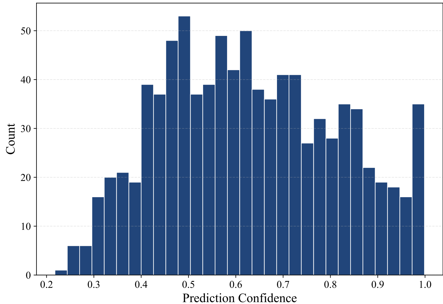
Prediction Confidence Distribution — Test Set
