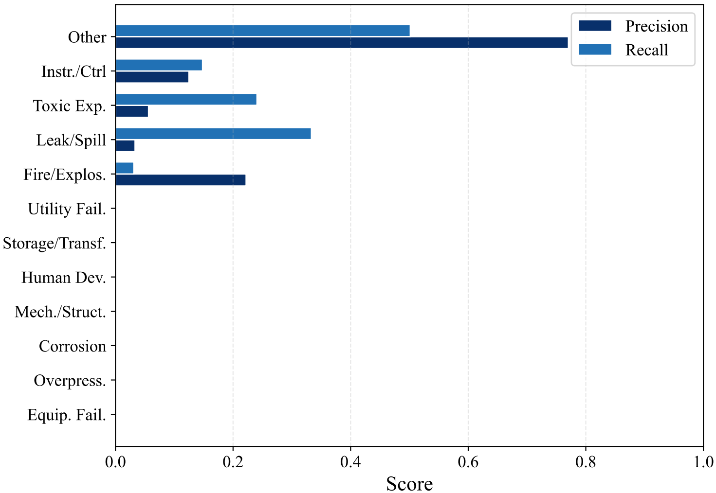
Per-Class Precision vs Recall — Test Set
