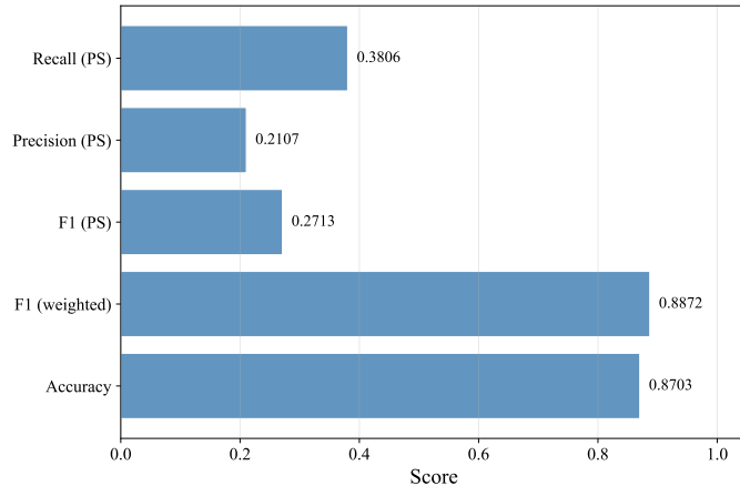
(b) Per-Class Metrics.
