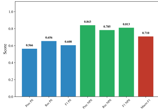
Classification Metrics — ENGLISH_MANUAL (bert-base-multilingual-uncased, SVM)
