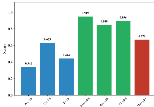
Classification Metrics — GERMAN_MANUAL (intfloat/multilingual-e5-large-instruct, SVM)
