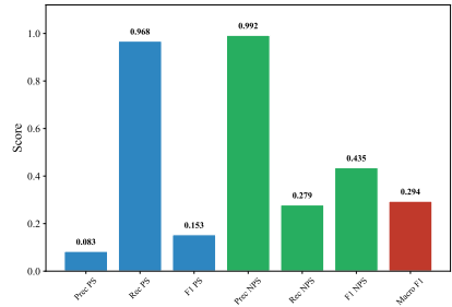
(b) Per-Class Metrics.
