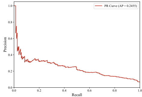
(c) Precision-Recall Curve.
