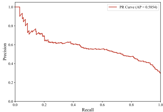
(c) Precision-Recall Curve.
