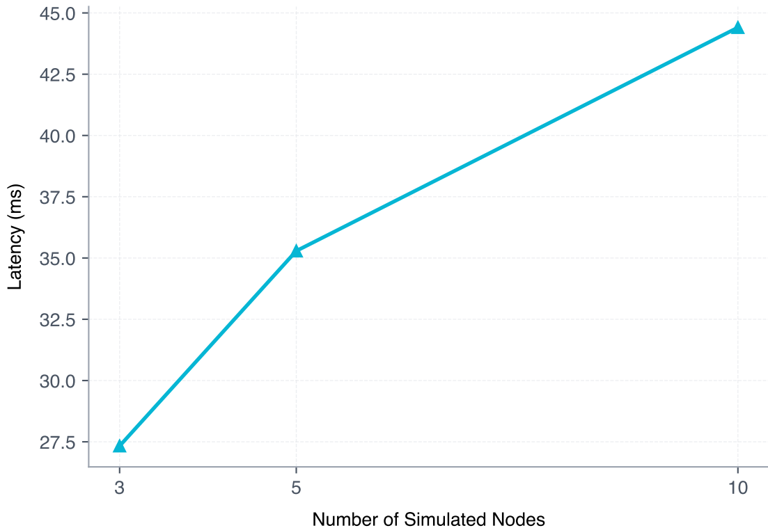
Heartbeat Latency vs. Node Scale
