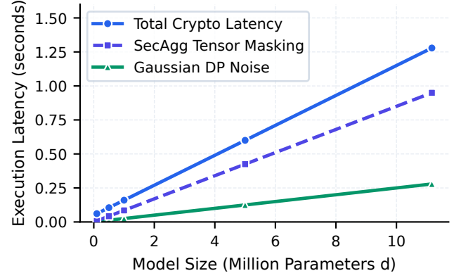
Fig. 11. Governance control plane latency and aggregation scaling across parameter dimensions for the PyTorch ResNet-18 deep learning architecture.
