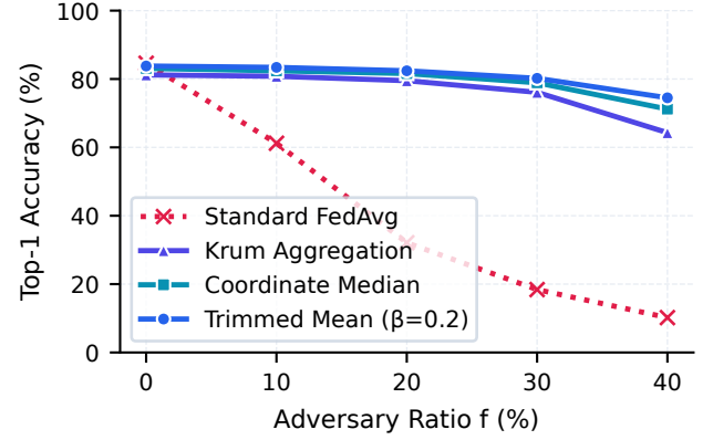
Fig. 8. Global accuracy degradation vs. Byzantine malicious client fraction f \in [0\%, 40\%] , demonstrating Trimmed Mean robustness under extreme poisoning.
