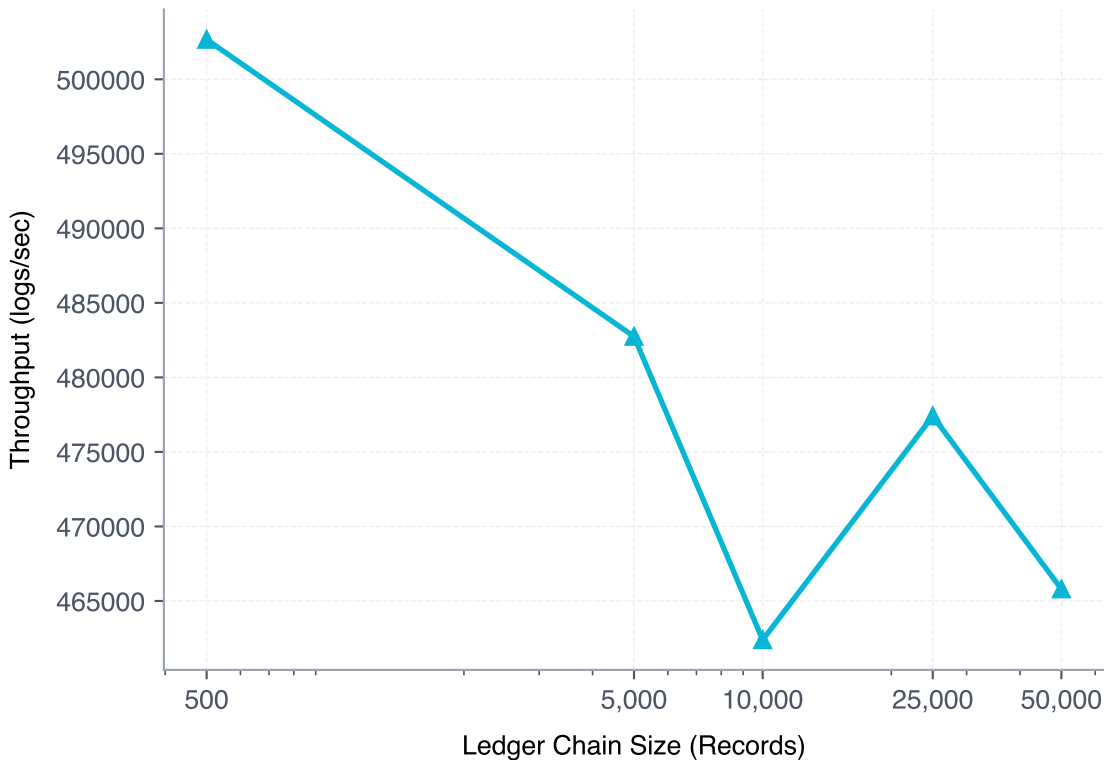
Verification Throughput vs. Chain Size
