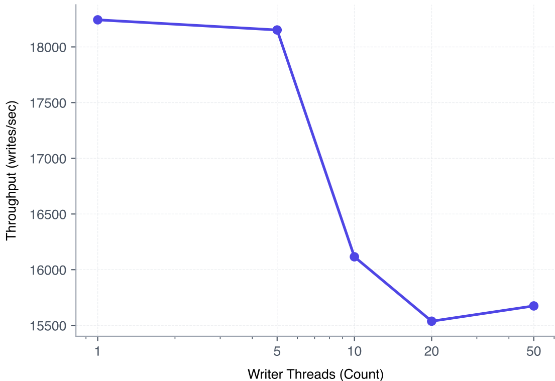
Ingestion Throughput vs. Threads
