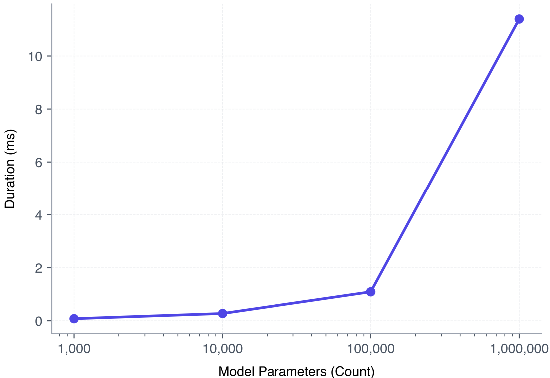
FedAvg Aggregation Time vs. Model Size
