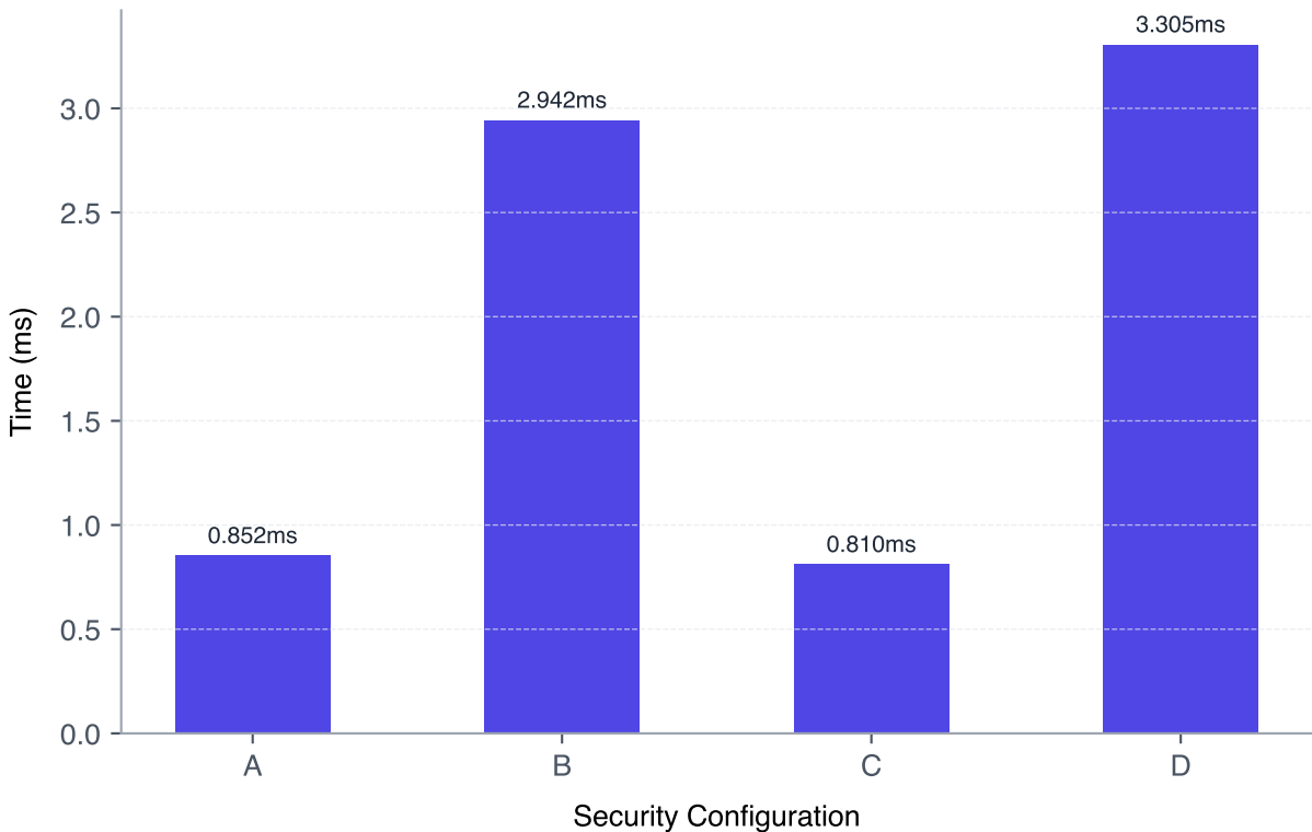
FedAvg Aggregation Time by Config
