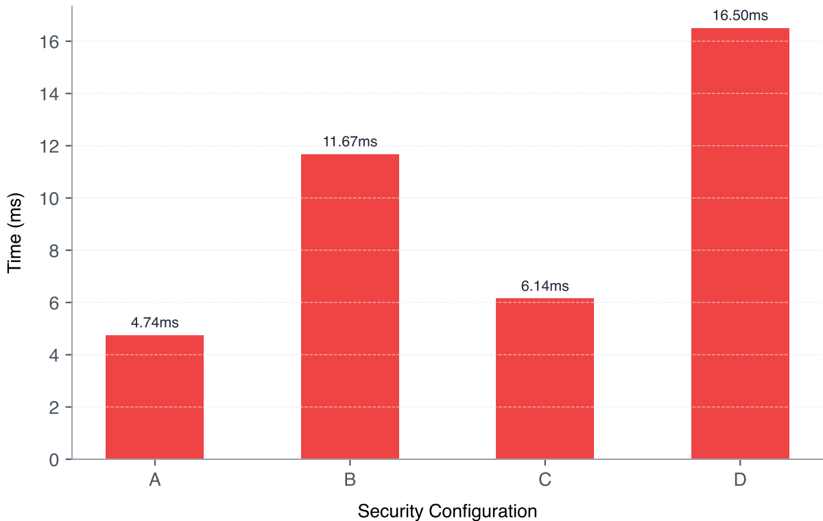
Total FL Round Duration by Config
