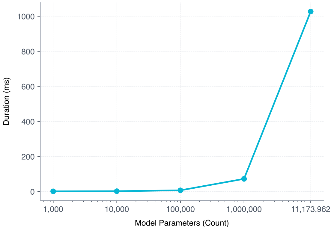
Secure Aggregation Time vs. Model Size
