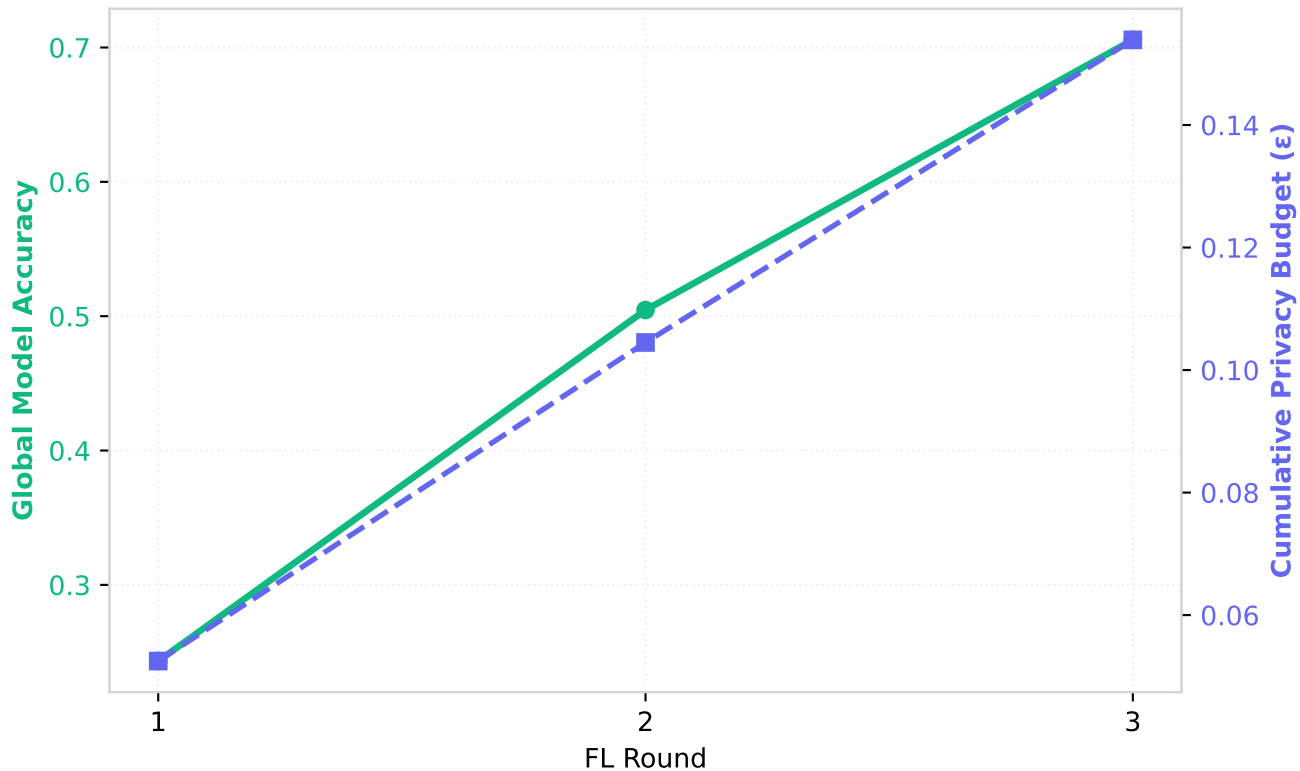
ResNet-18 Accuracy Trajectory vs. Cumulative Rényi DP Consumption
