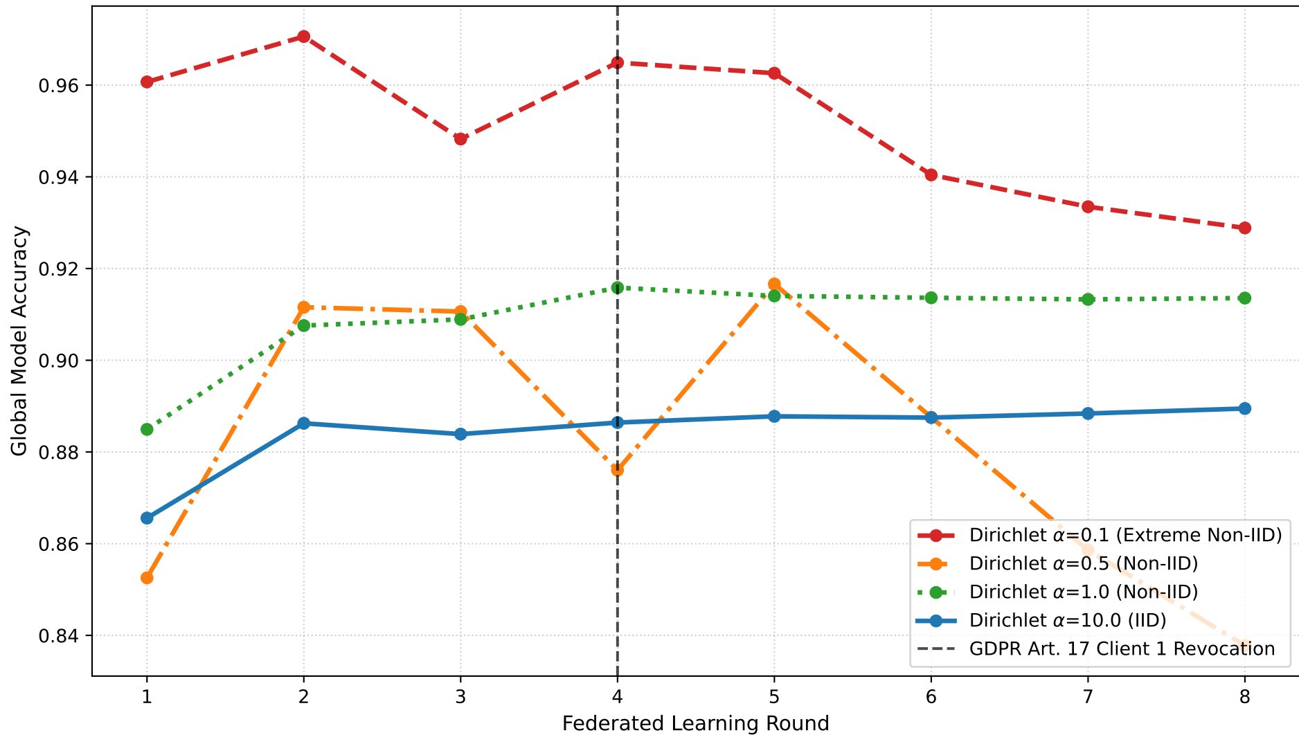
Conclave: Model Accuracy Trajectories under Dirichlet Skew & GDPR Art. 17 Revocation
