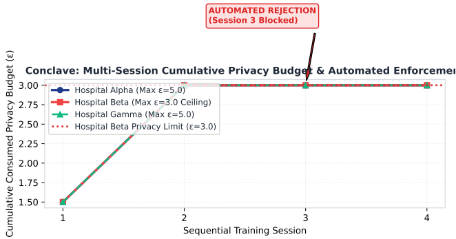
Fig. 4. Cumulative differential privacy budget consumption ( \epsilon ) across federated training rounds for \delta = 10^{-5} , C = 1.0 , \sigma = 0.85 , illustrating dynamic privacy threshold enforcement.
