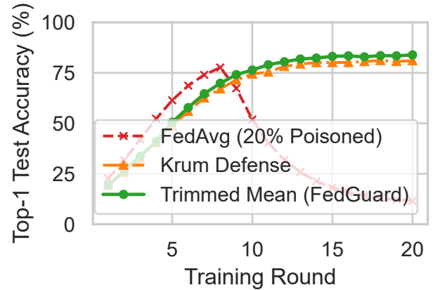
Fig. 9. Global model test accuracy over training rounds under Byzantine gradient poisoning, comparing standard Federated Averaging (FedAvg) against FedGuard with Byzantine-robust aggregation primitives.
