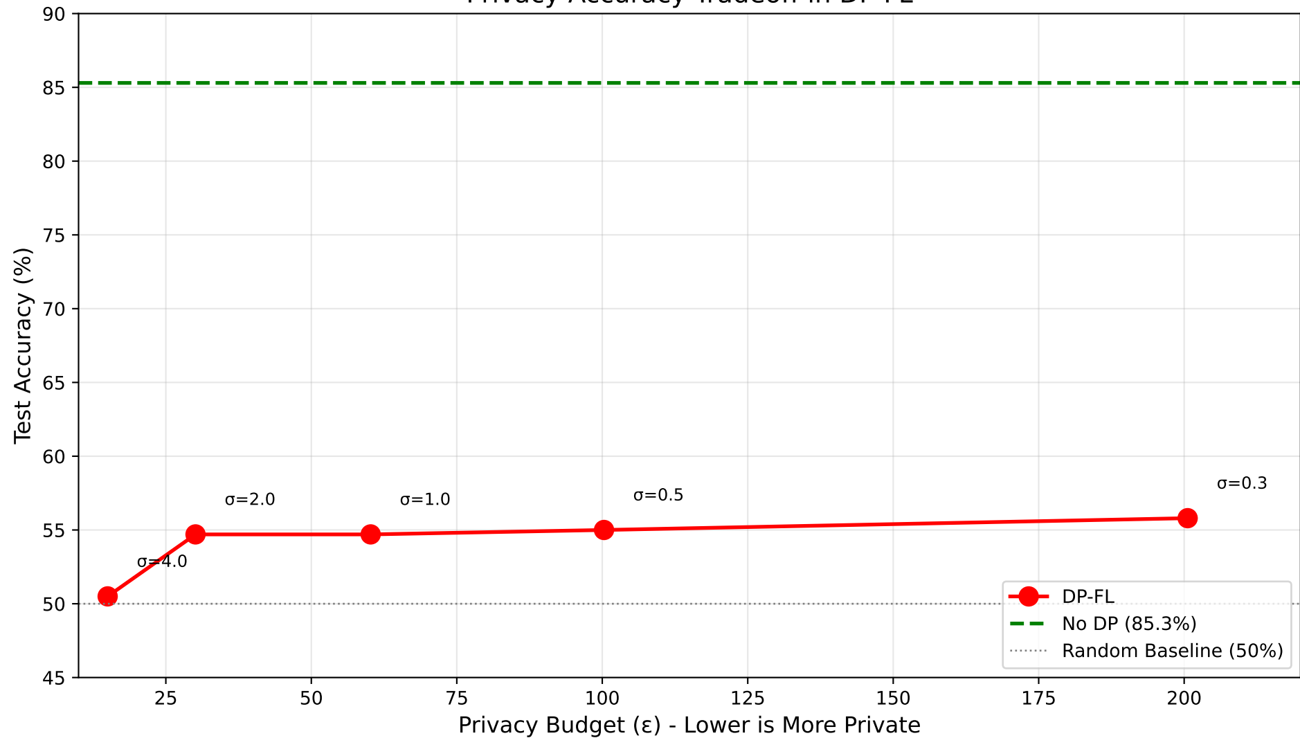
Privacy-Accuracy Tradeoff in DP-FL
