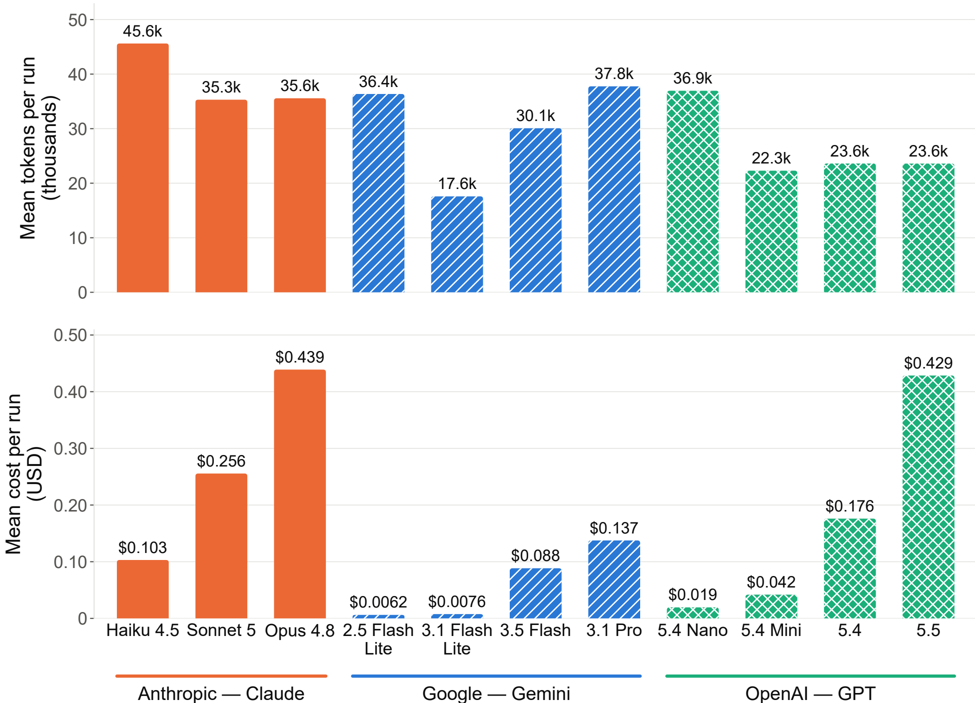
Mean token usage and cost per run, by model
