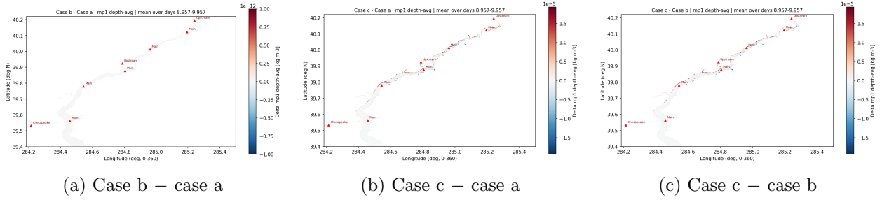
Figure 5: Day-mean depth-averaged mp1 difference maps [kg m -3 ], final 24 h of the 10-day run. Diverging colour scale (red = gain, blue = loss). b-a : near-zero everywhere — cases a and b are identical ( D_{50} = 0.1 mm, no aggregation). c-a and c-b : case c shows elevated concentrations near river mouths (stronger local aggregation) and reduced concentrations further downstream (faster bed removal).
