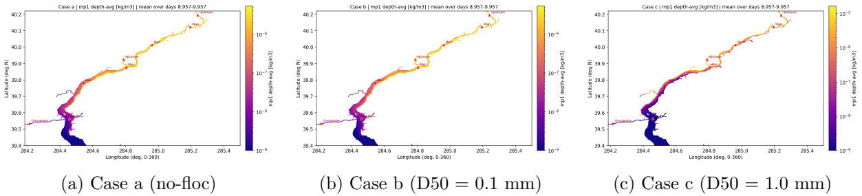
Figure 1: Day-mean depth-averaged mp1 concentration [ \text{kg m}^{-3} ], final 24 h of the 10-day run. Log colour scale. Cases a and b are visually identical (peak 1.7 \times 10^{-4} \text{ kg m}^{-3} ). Case c peak is 3.7 \times 10^{-3} \text{ kg m}^{-3} ( \approx 21\times higher) due to active aggregation and altered settling.
