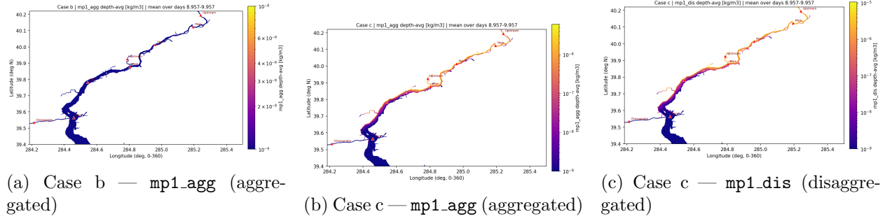
Figure 2: Day-mean depth-averaged aggregated (mp1_agg) and disaggregated (mp1_dis) fractions, final 24 h of the 10-day run. Case b: mp1_agg = 0 everywhere (fine sediment, D50 = 0.1 mm — weak heteroaggregation kinetics). Case c: mp1_agg reaches 1.1 \times 10^{-3} \text{ kg m}^{-3} and is non-zero across most of the domain; mp1_dis mirrors the overall plume.
