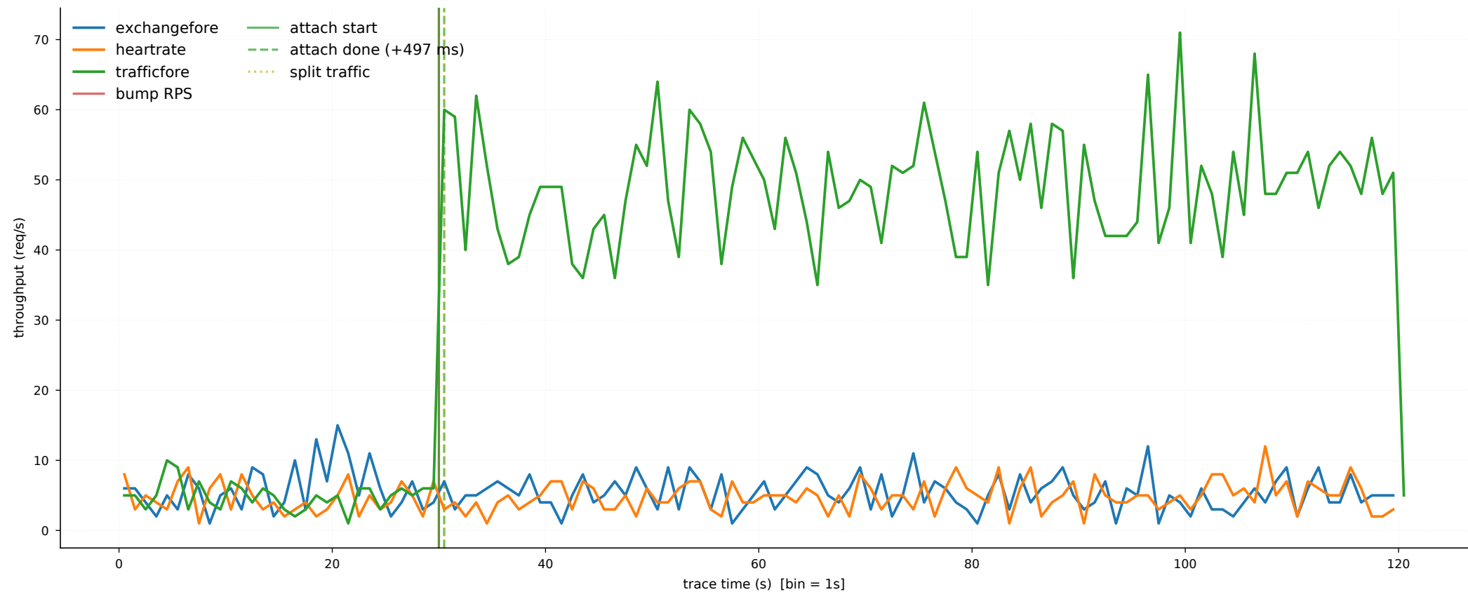
Per-task throughput vs. time (case1)
