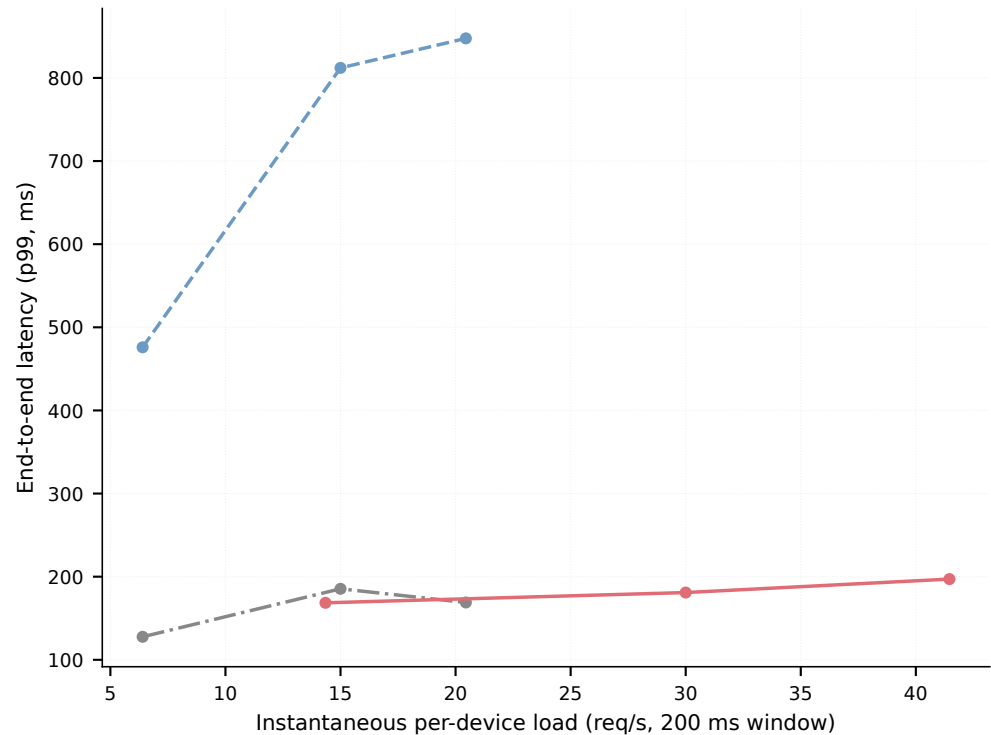
p99 latency vs load (N=16)
