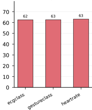
Sharing (STFQ)
