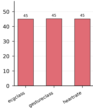
Sharing (STFQ)
