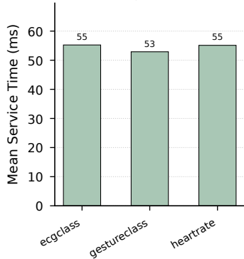
Single Task
