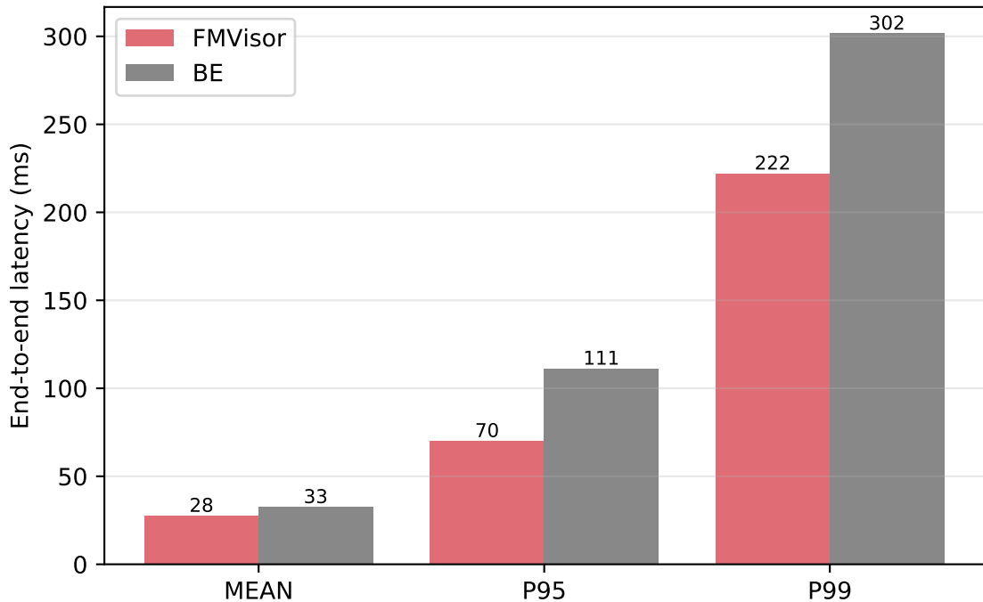
mix_L35_M30_H20: response-time summary
