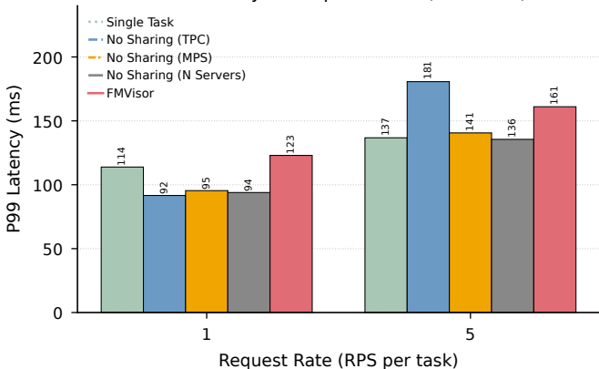
P99 Latency vs Request Rate (ntasks=2)
