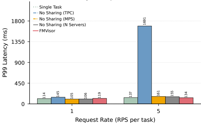
P99 Latency vs Request Rate (ntasks=3)
