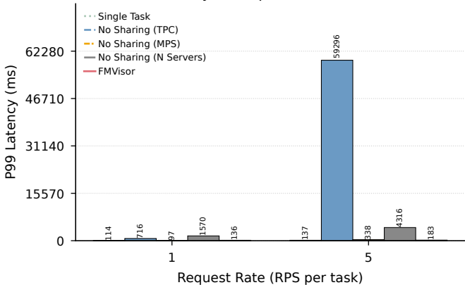
P99 Latency vs Request Rate (ntasks=5)
