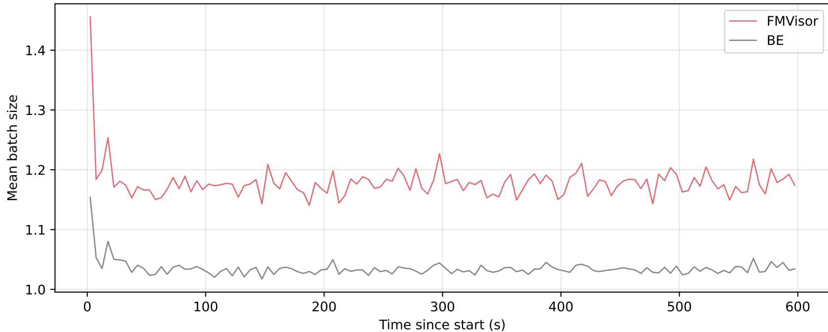
mix_L35_M30_H20: mean batch size over time (bin=5s)
