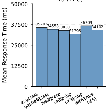
NS (TPC)
