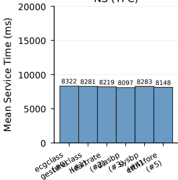
NS (TPC)
