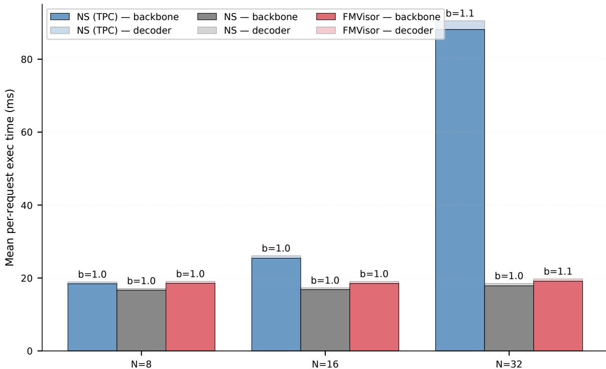
Backbone vs decoder exec time (b = request-weighted batch size)
