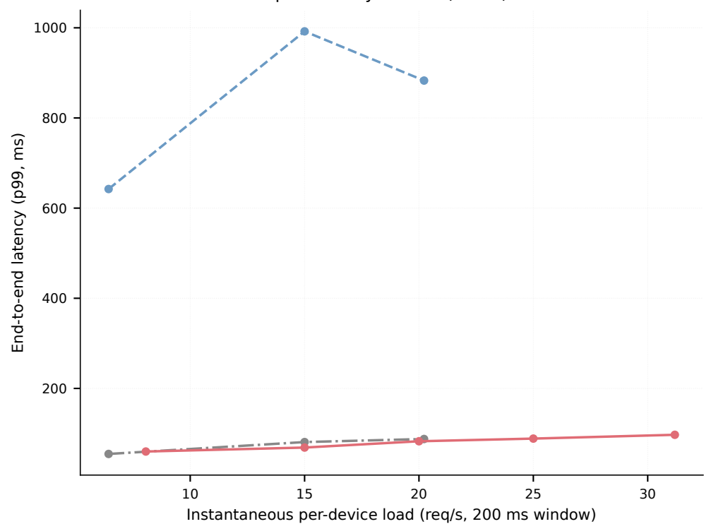
p99 latency vs load (N=32)
