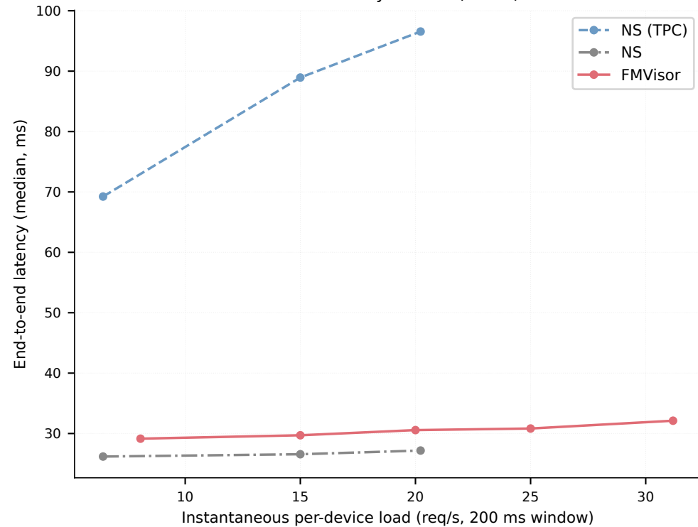
Median latency vs load (N=32)
