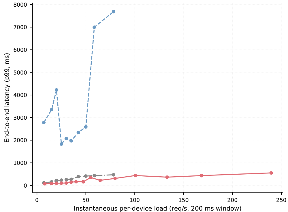
p99 latency vs load (N=32)
