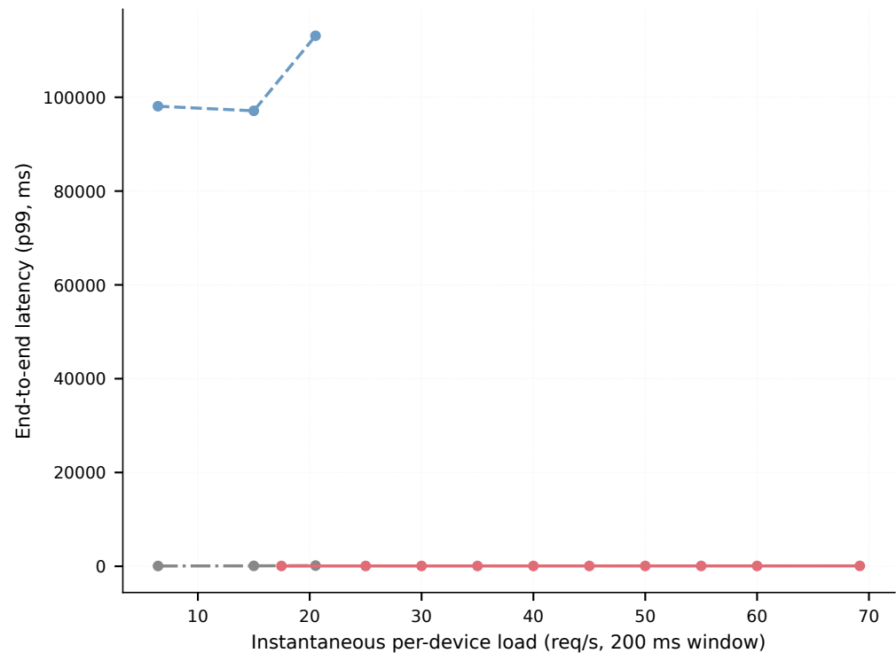
p99 latency vs load (N=64)
