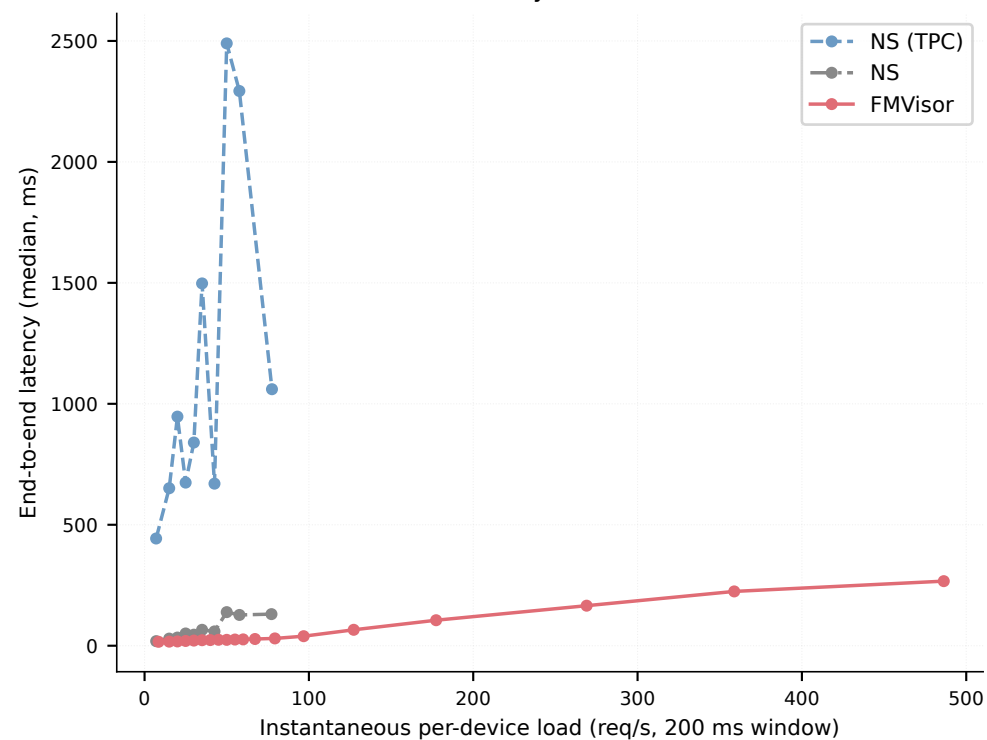
Median latency vs load (N=64)
