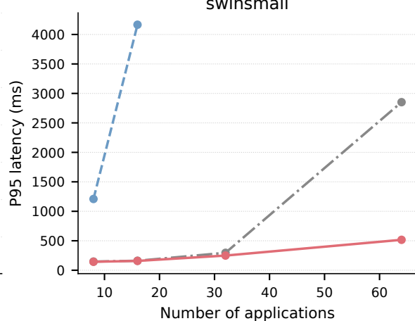
swinsmall
