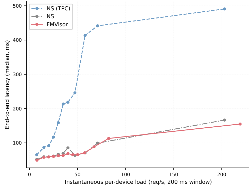
Median latency vs load (N=16)
