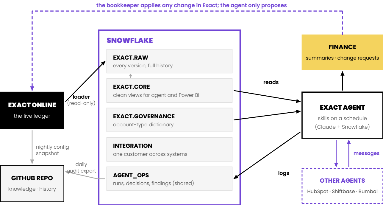
Figure 3. Data flow. Exact data lands in Snowflake; the agent reads and logs there; any change in Exact is made by the bookkeeper and confirmed by the next load.
