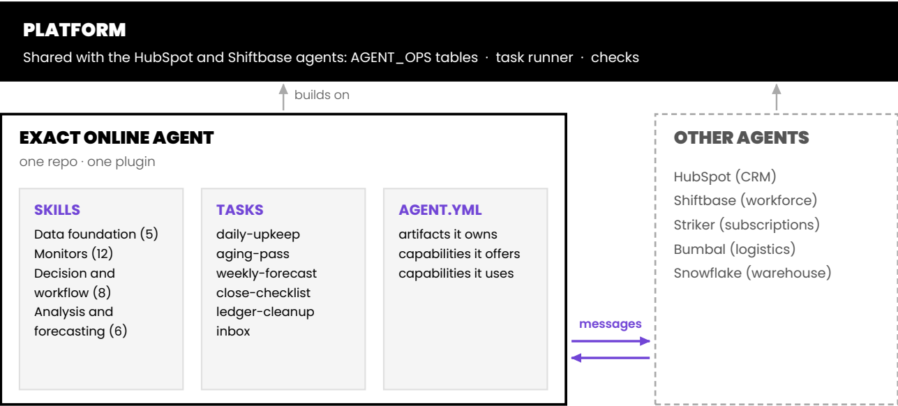
Figure 2. The hierarchy. The platform is shared by all agents; the Exact Online agent is its own repository and plugin; agents cooperate only through messages.
