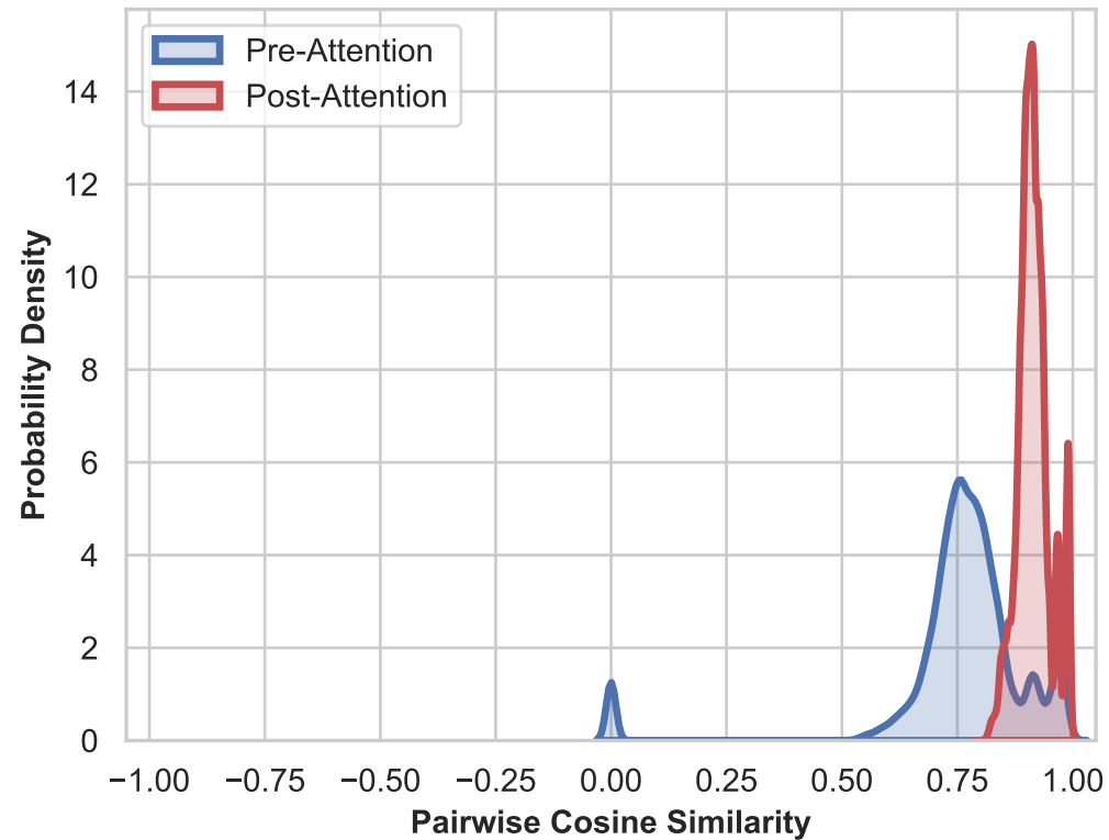
A. Token Homogenization Distribution
