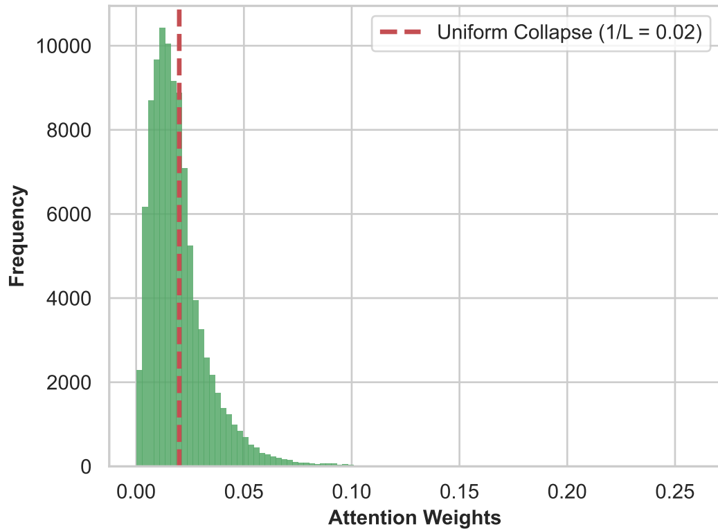
B. Cross-Attention Softmax Collapse
